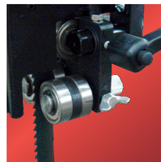
Adjustable 5-point ball bearing guides
