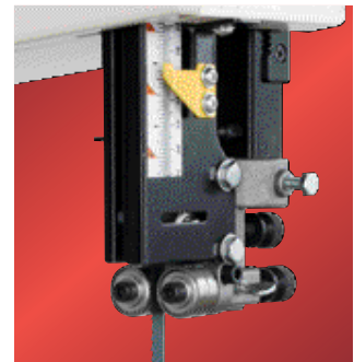
Upper and lower precision roller guide
