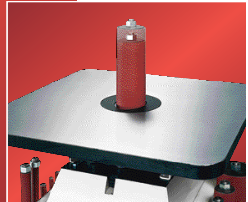
38 mm spindle stroke, table tilts 45°
