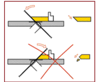
Advantages of tilting to the left: Cleaner cut from above. No collision with fence. Workpiece cannot get jammed when cutting at the fence.
