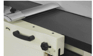
Eccentric rapid adjustment of the infeed table
