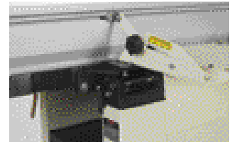
Double guided jointing fence, tilts at the table
