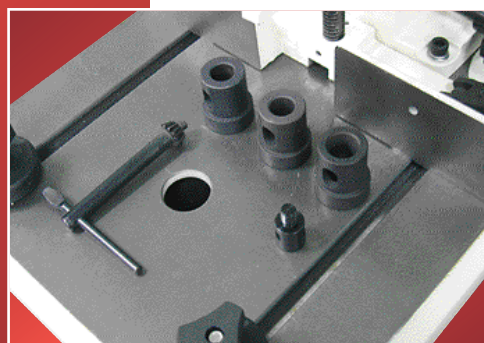
Chisel shank adapters \frac{5}{8} " , \frac{3}{4} " , \frac{13}{16} " , long chuck key and spindle extension standard
