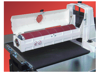
Quick and simple system to fix the abrasive strips
