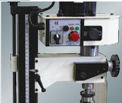
Variable speed control with right/left-handed rotation and 2-step gear box
