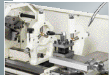
Steady rest and follow rest
