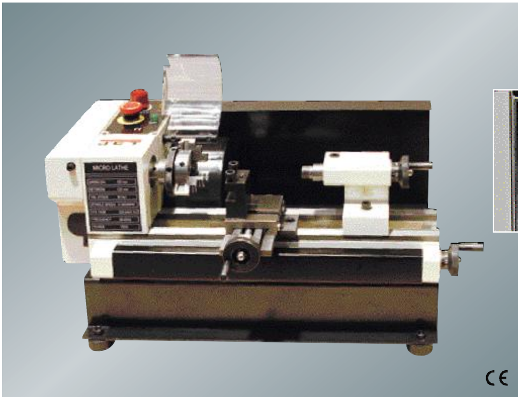
Variable speed range 100–3800 rpm
